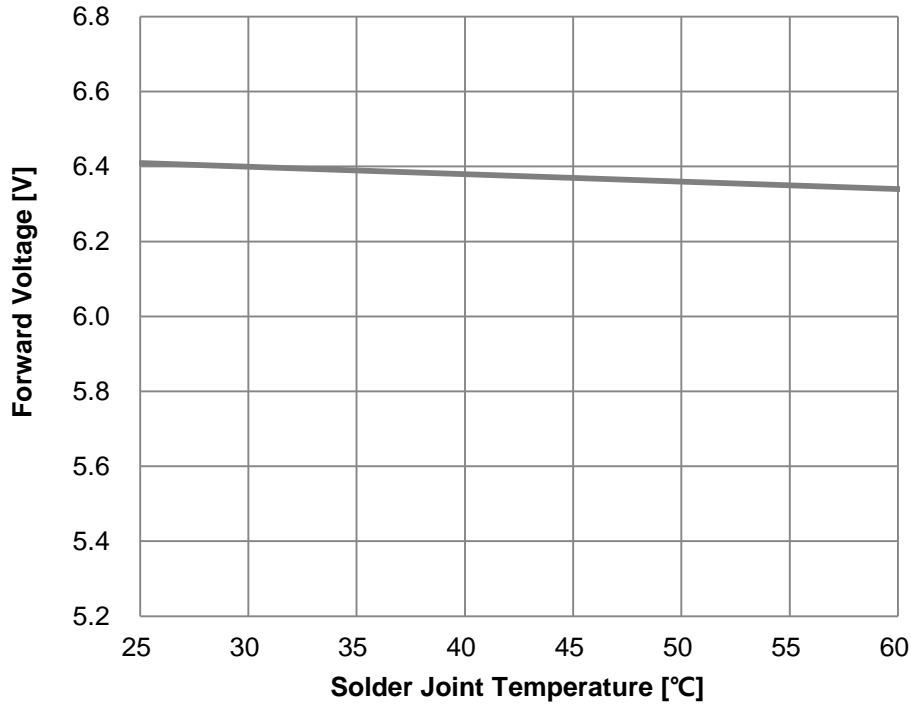
Fig 7. Solder Joint Temperature vs. Forward Voltage, I_F=600\text{mA}
