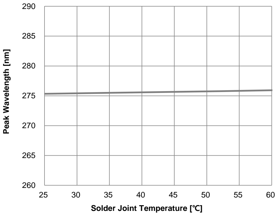
Fig 6. Solder Joint Temperature vs. Peak Wavelength, I_F=600\text{mA}
