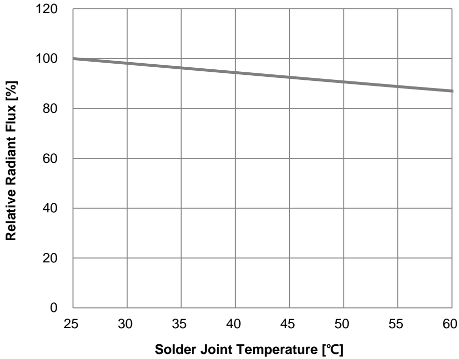
Fig 5. Solder Joint Temperature vs. Relative Radiant Flux, I_F=600\text{mA}
