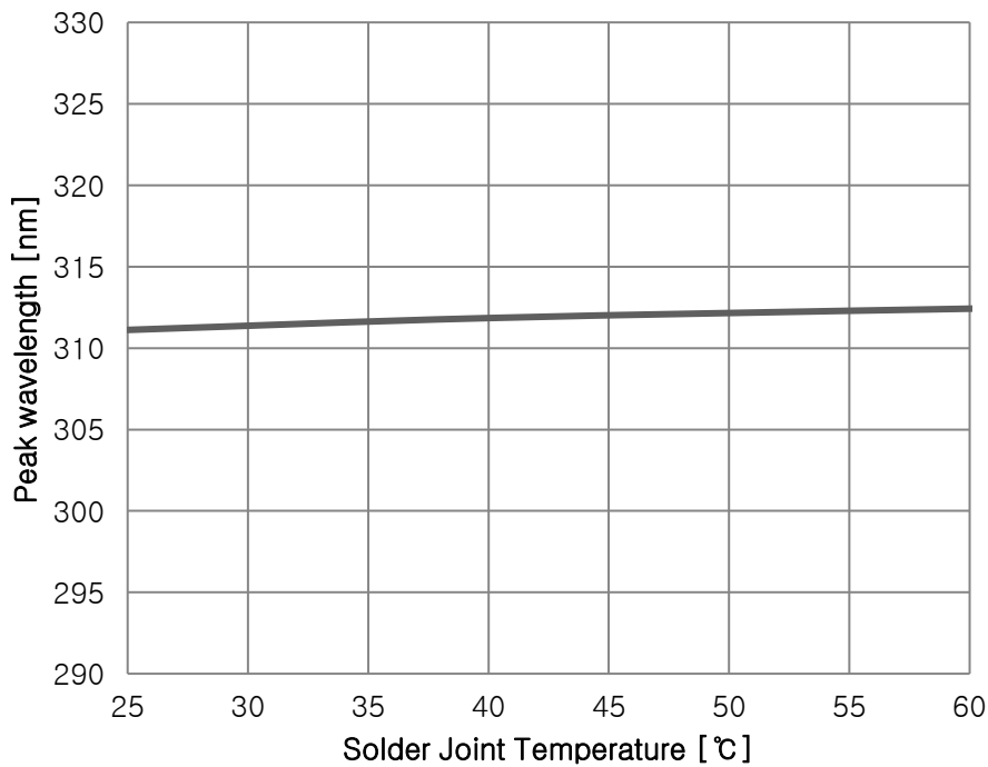
Fig 6. Surface Temperature vs. Peak Wavelength, I_F=20mA
