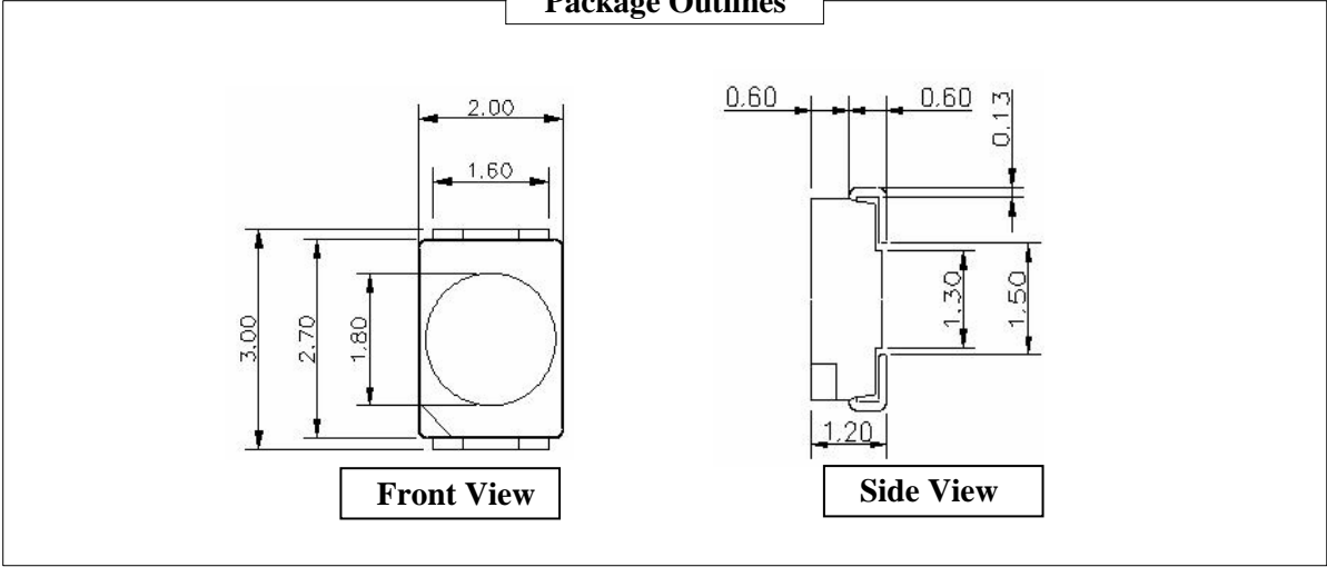
Package Outlines
