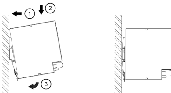
Fig. 3.1 Mounting
