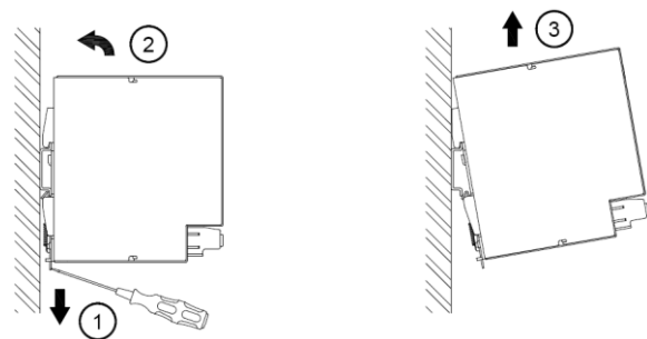
Fig. 3.2 Dismounting
